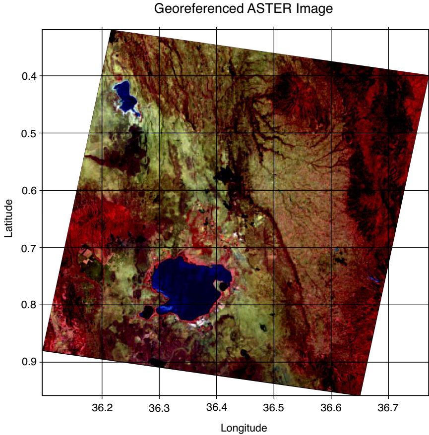
Fig. 8.5 Georeferenced RGB composite of an TERRA-ASTER image using the infrared bands v Nir_Band3n , 2 and 1. The result is displayed using imshow . Original image courtesy of NASA/GSFC/METI/ERSDAC/JAROS and U.S./Japan ASTER Science Team.
