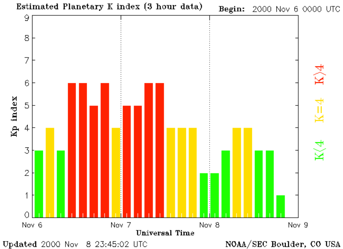
Figure 6-2 K-Index for 07-09 November 2000
